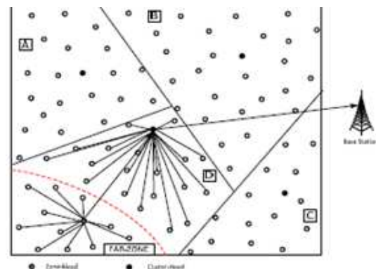
Fig 3. Communication within and from Far-Zone.
